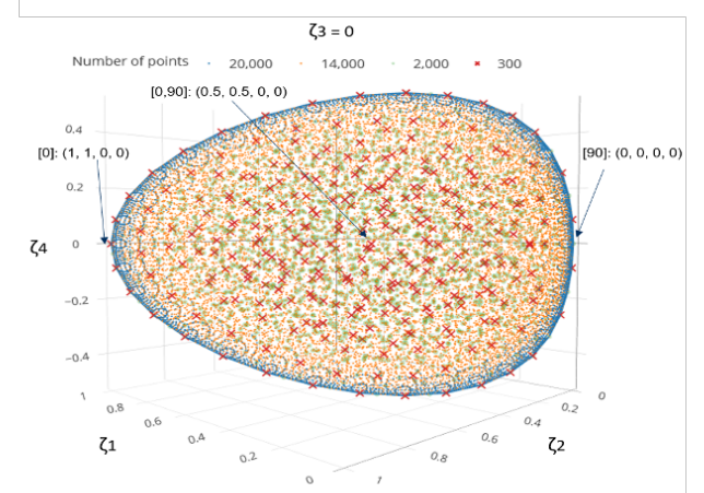
Feasible lamination parameters space (z1, z2, z3, z4). Projection with z3 = 0. Four levels of simplification (20,000 - blue to 300 points - red).
